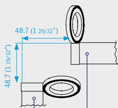
DC0720 (DC0820)
